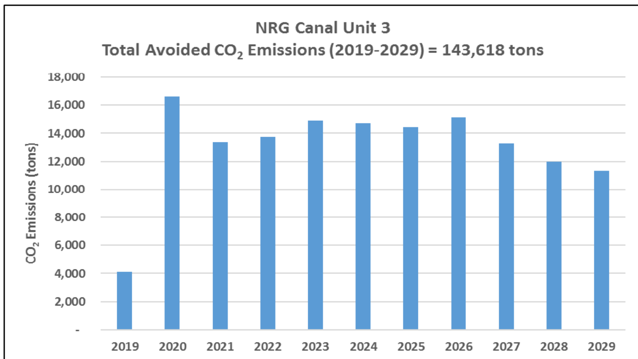
Figure DEP-10 Total Avoided CO 2 Emissions
