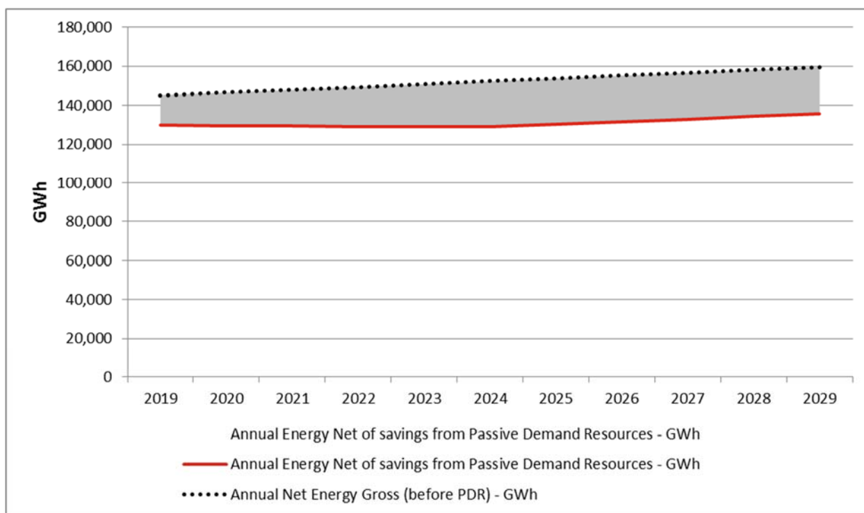
Figure 3. New England energy load – gross and net of EE
